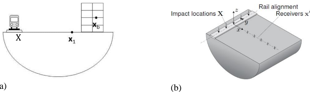
Figure 1: (a) Source, soil and receiver positions; (b) excitation and receiver locations for line source transfer mobility measurements.
