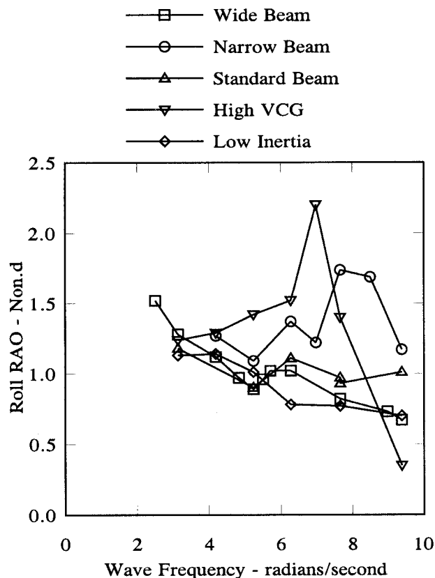
Figure 10. Roll RAOs for the catamaran models.
