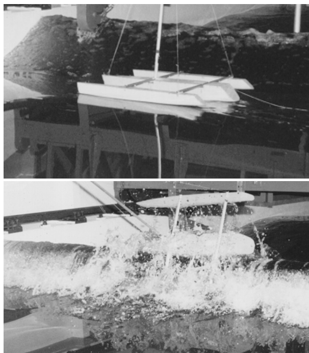
Figure 11. Photographs of a test on the trimaran with large floats in a breaking wave.
