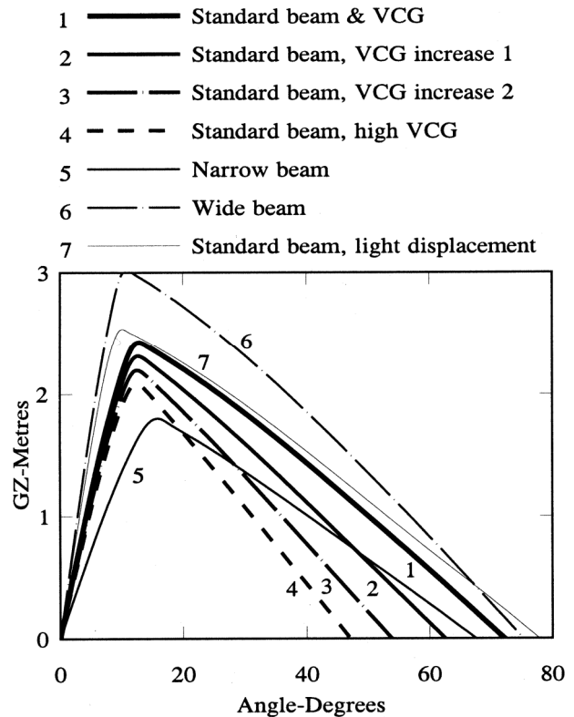
Figure 9. Stability curves for the catamaran models used for the roll tests.
