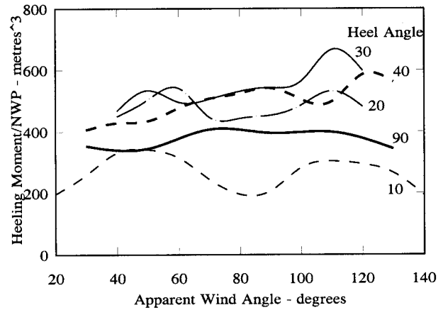
Figure 4. Wind heeling moments in configuration 2 at selected heel angles.
