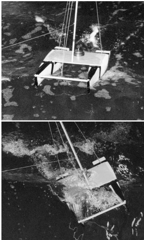
Figure 12. Two photographs from a pitchpoling test on the fine bow catamaran.
